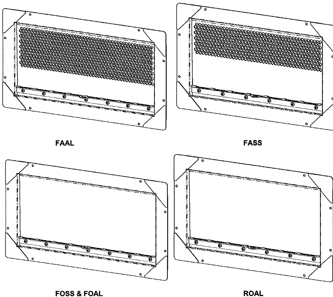
FIGURE 1—USA FLOOD AIR VENTS
